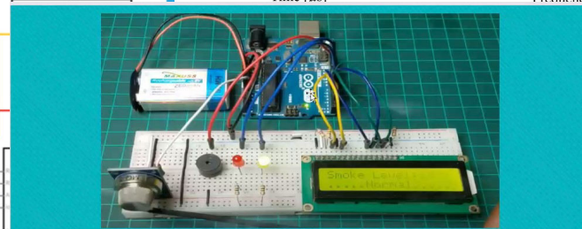
4. Prototype of gas detector system.
